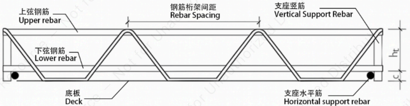
Structural Diagram
